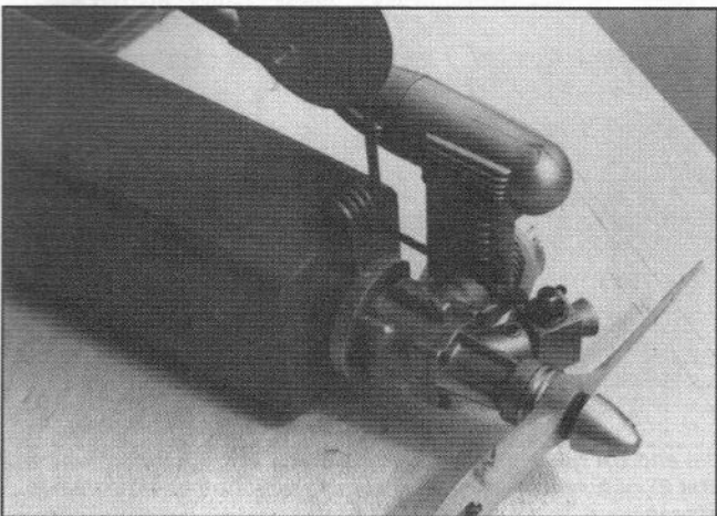
K&B 40 mounted using Bill Evans E-Z mount.
