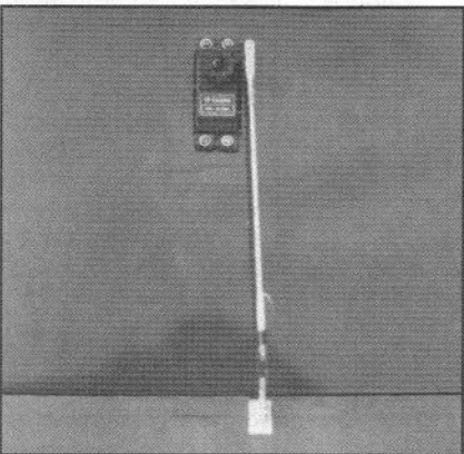
Servo mounted on bottom of wing. One is used on each elevon with electronic mixing.
