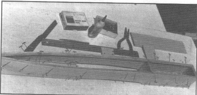
After fuselage sides are joined and CA'ed at rear, pin top 1/4" sq. longerons in place and CA them.
