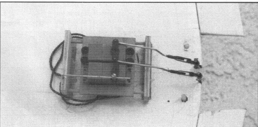
Example of sliding tray system which can be used to effect mechanical elevon mixing.
