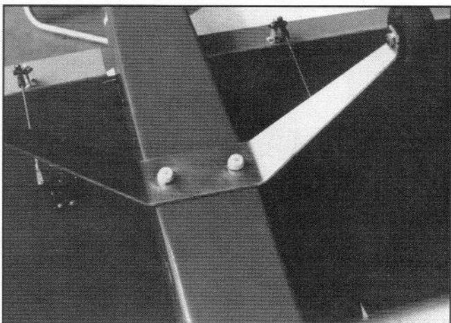
Landing gear is mounted, using 10-32 nylon bolts.
