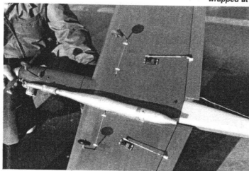
Bottom view showing pipe and elevon servos mounted in wing.
