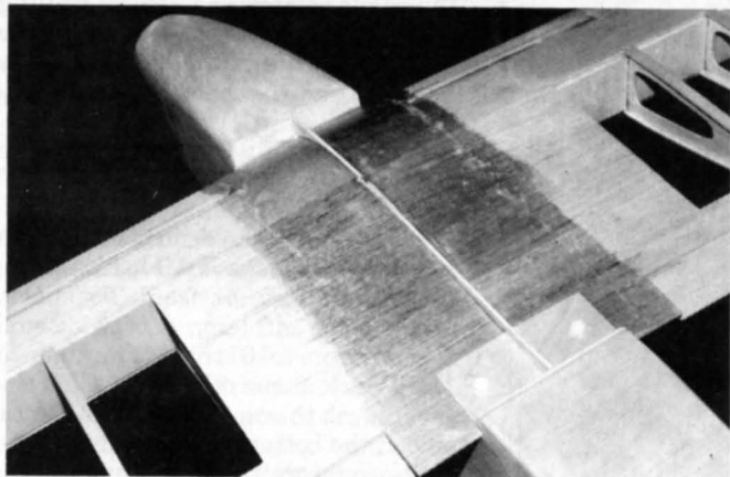
Formers and spine are used to guide the shaping of the wing fairings.
